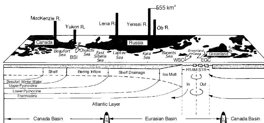
Schematic drawing of circulation and stratification patterns associated with river inflow and halocline ventilation in the Arctic Ocean (modified from Carmack, 1990). Shown is river runoff scaled to average annual discharge of 555 km 3 of the Yenisei river.
