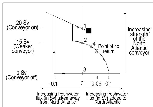
Schematic diagram showing the behavior of the North Atlantic Conveyor as freshwater perturbation is slowly varied (Weaver, 1995).
